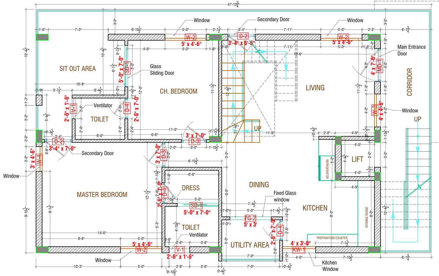
SECOND FLOOR BRICK MARKING PLAN
